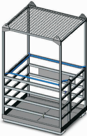
(Lifting Chains not shown)
