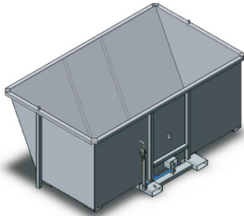
(Type NS-JTU-18 standard model shown) Refer 'NS-JTU_WL_Sales' Product Specification sheet for Wheels & Crane Lug options.
